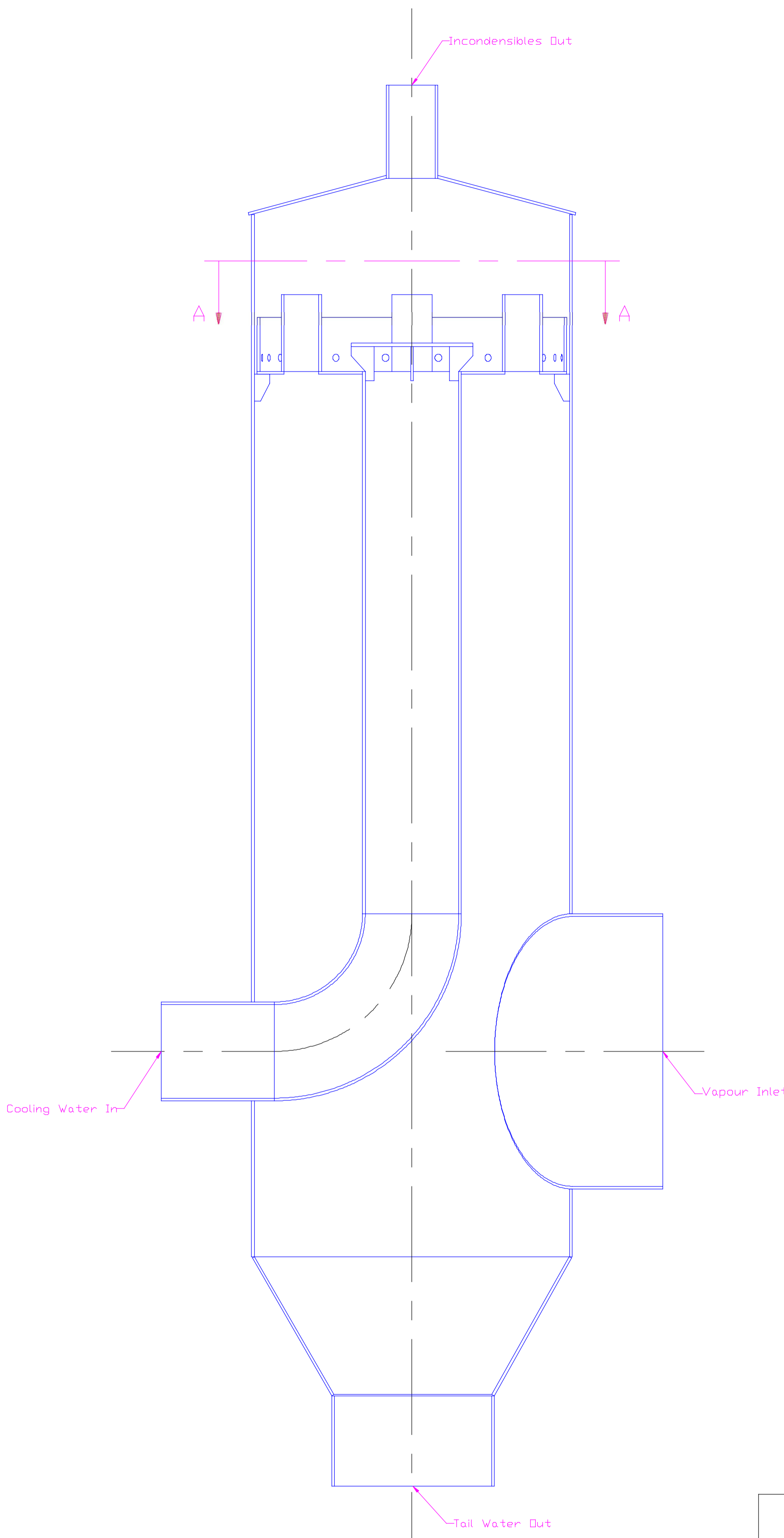
Sectional Elevation
